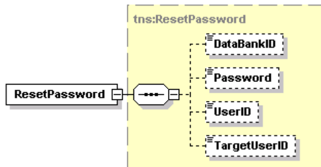
Figure 11 - ResetPassword
